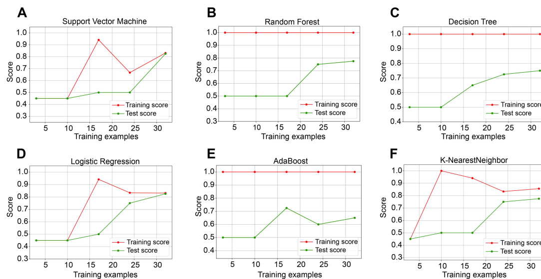
(A) Learning curve analysis of the SVM classifier. (B) Learning curve analysis of the RF classifier. (C) Learning curve analysis of the DT classifier. (D) Learning curve analysis of the LR classifier. (E) Learning curve analysis of the ADA classifier. (F) Learning curve analysis of the KNN classifier.
