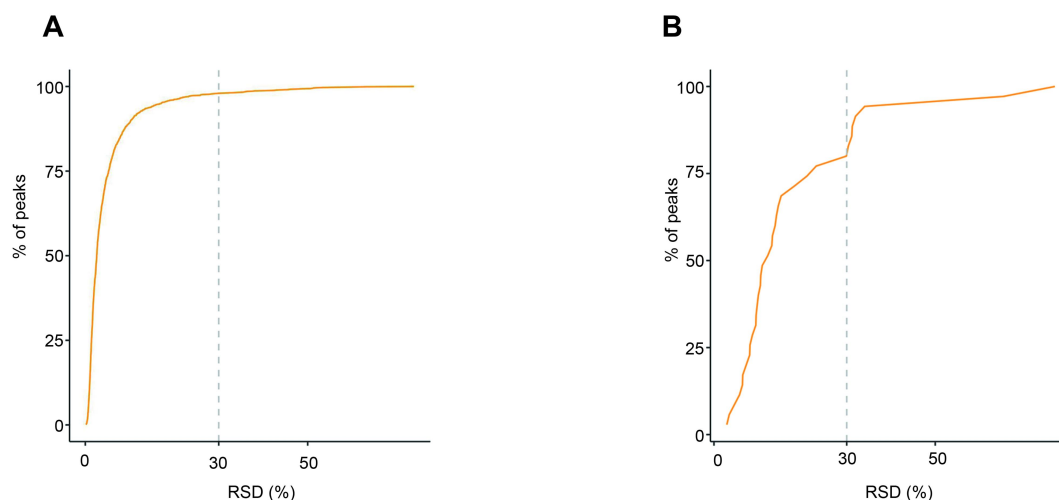
(A) QC RSD distribution of quality control samples in the untargeted lipidomics. (B) QC RSD distribution of quality control samples in the targeted lipidomics.
