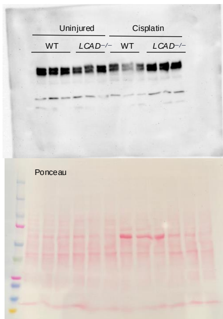
Figure 8D (PEX5)
