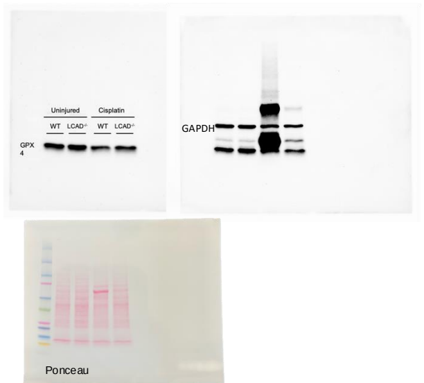
Figure 9D (GPX4)
