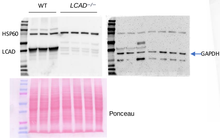
Figure 1A (LCAD)
